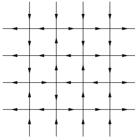
Fig. 2. An example of 4 \times 4 configuration
