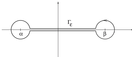
Fig. 8. The contour \Gamma_\varepsilon
