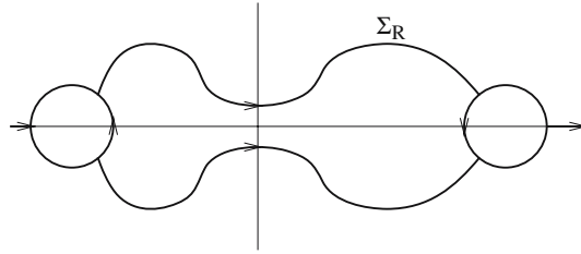
Fig. 7. The contour \Sigma_R
