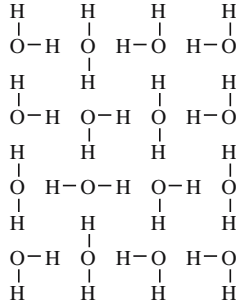
Fig. 3. The corresponding ice model
