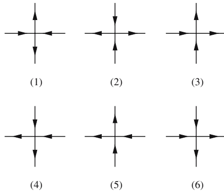
Fig. 1. The six arrow configurations allowed at a vertex
