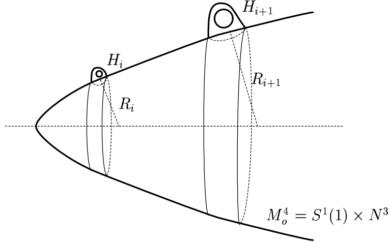
Figure 10: The 4D Sha-Yang Example with p = 2 and q = 2
