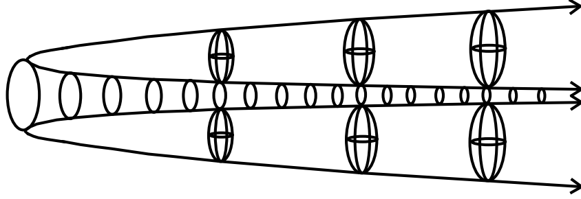
Figure 2: Nabonnand's Example
