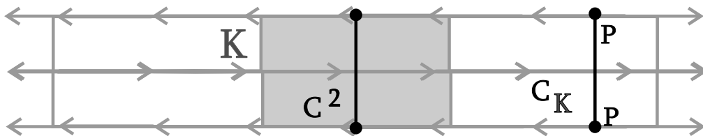
Figure 5: An infinite Moebius strip, defined as \mathbb{E}^2 with points (x, y) identified with (-x, y + 1) , also fails to have the loops to infinity property.
