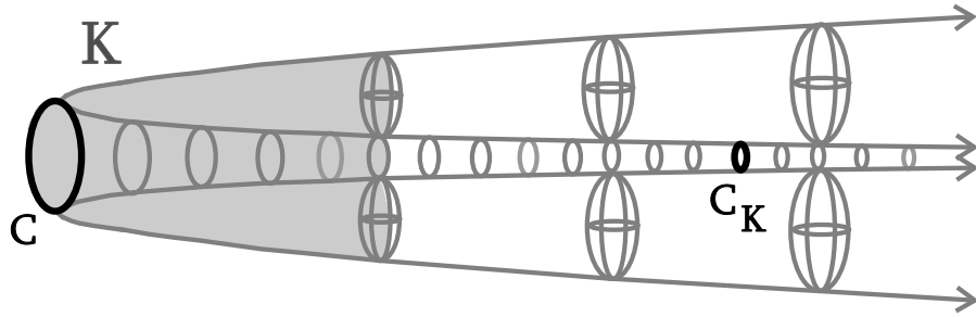
Figure 3: Nabonnand's example has the loops to infinity property as can be seen taking the shaded compact set K .
