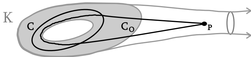
Figure 3: Nabonnand's example has the loops to infinity property as can be seen taking the shaded compact set K .
