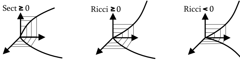
Figure 1: The bending of geodesics under curvature bounds.
