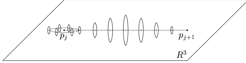
Figure 11: Anderson-Kronheimer-LeBrun Example
