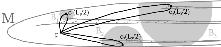
Figure 8: Halfway generators: c_i satisfy (3.11), c does not.
