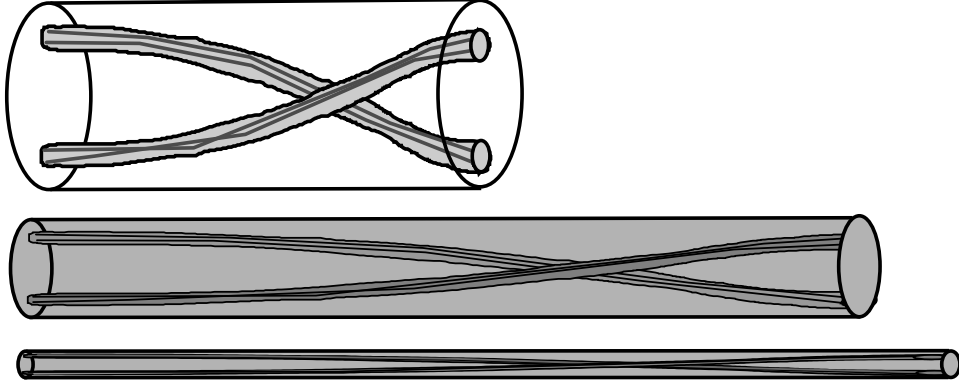
Figure 13: Constructing the Dyadic Solenoid Complement
