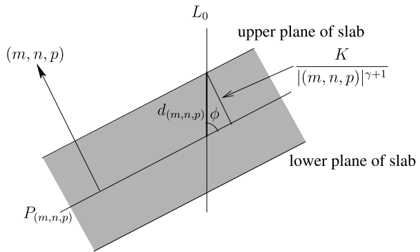
Fig. 5 The intersection of the line segment L_0 and the slab S_{(m,n,p)}
