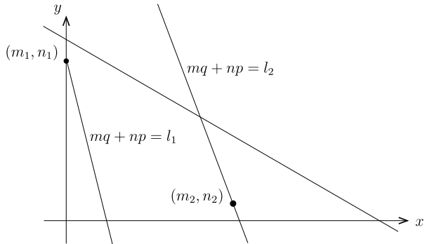
Fig. 3 The points (m_1, n_1) and (m_2, n_2) on lines mq + np = l_1 and mq + np = l_2
