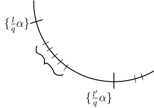
FIGURE 4. Points with first component \frac{l}{q}\alpha
