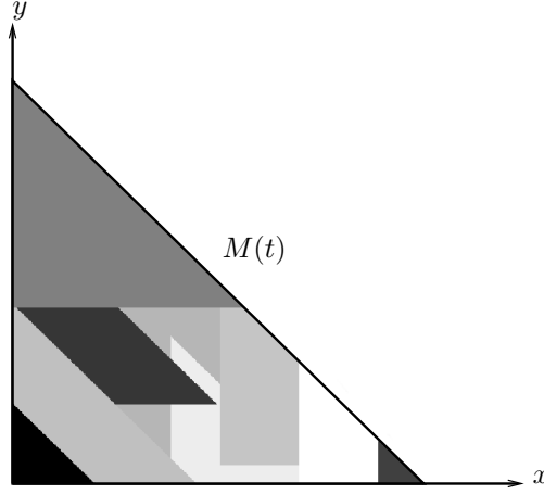
FIGURE 1. The partition \{M_k(t)\} of M(t) for \boldsymbol{\omega} = (\sqrt[3]{2}, \sqrt[3]{4}) and t = 650 .
